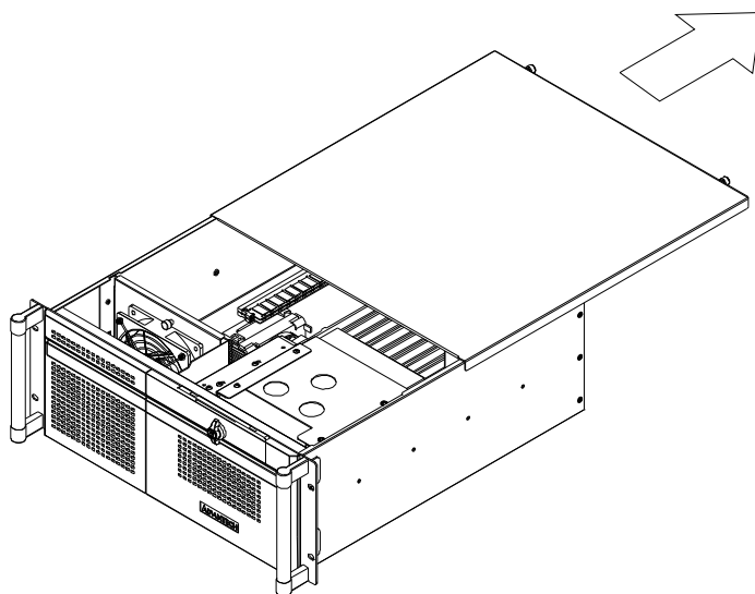
Figure 2.1 Removing the Top Cover/ 移除顶盖 / 移除上盖
