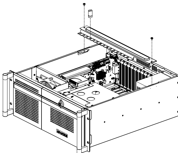
Figure 2.6 Installing Rubber Cushions and Hold-down Clamp/ 安装橡胶垫和固定压条 / 安裝橡膠墊和壓桿
