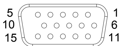
Figure 2.17 VGA Connector
