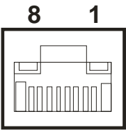
Figure 2.9 Ethernet Connector
