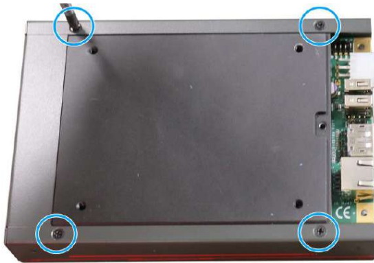
Screws holding the flattop heatsink with enclosure
