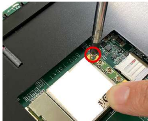
Secure the card with a screw
