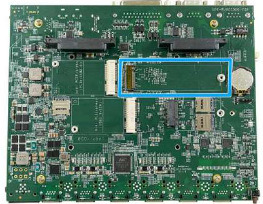
Location of M.2 M key socket (heat spreader removed)
