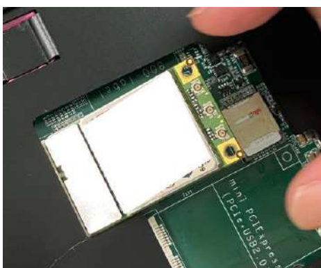
45 degree angle insert
