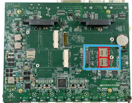
Location of M.2 B key and internal SIM card slot (heat spreader removed)
