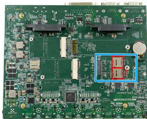
Location of M.2 B key and internal SIM card slot (heat spreader removed)
