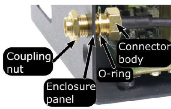
Secure the connector body, coupling nut onto a antenna opening on a panel
