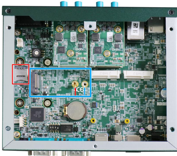
M.2 B key and internal SIM card slot
