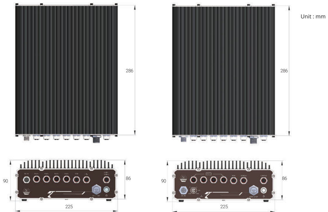
Nuvo-9650AWP
