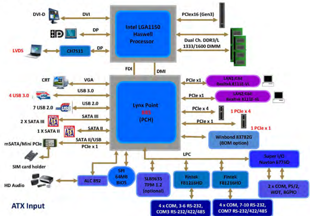
AIMB-503F-00A1E (B85)
