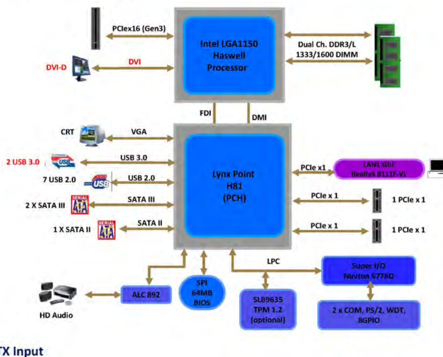
Figure 1.5 AIMB-503L Block Diagram
