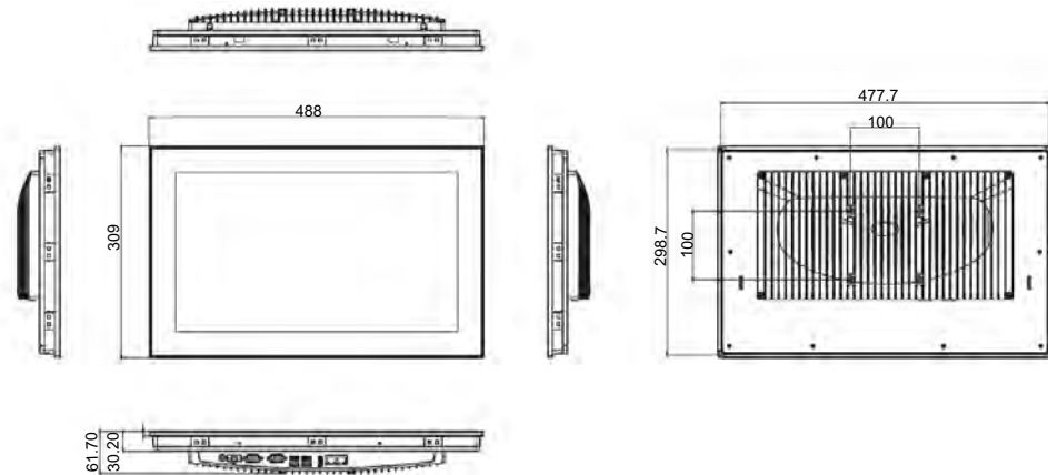
Figure 1.5 PPC-3181SW dimensions
