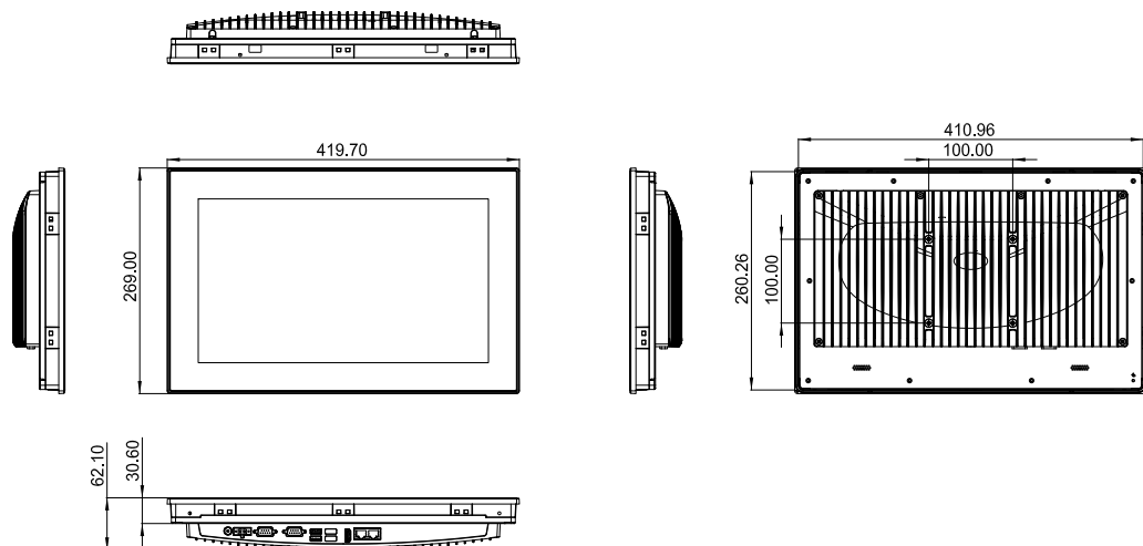
Figure 1.6 PPC-3151SW dimensions
