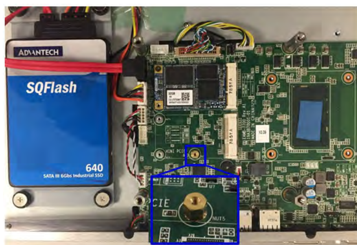
Figure 2.14 Hexagonal screw location
