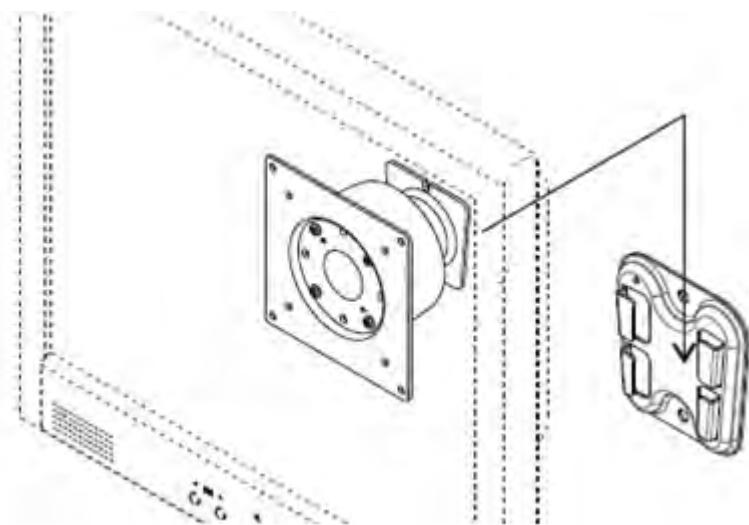
Figure 2.22 Mounting the panel PC on a wall
