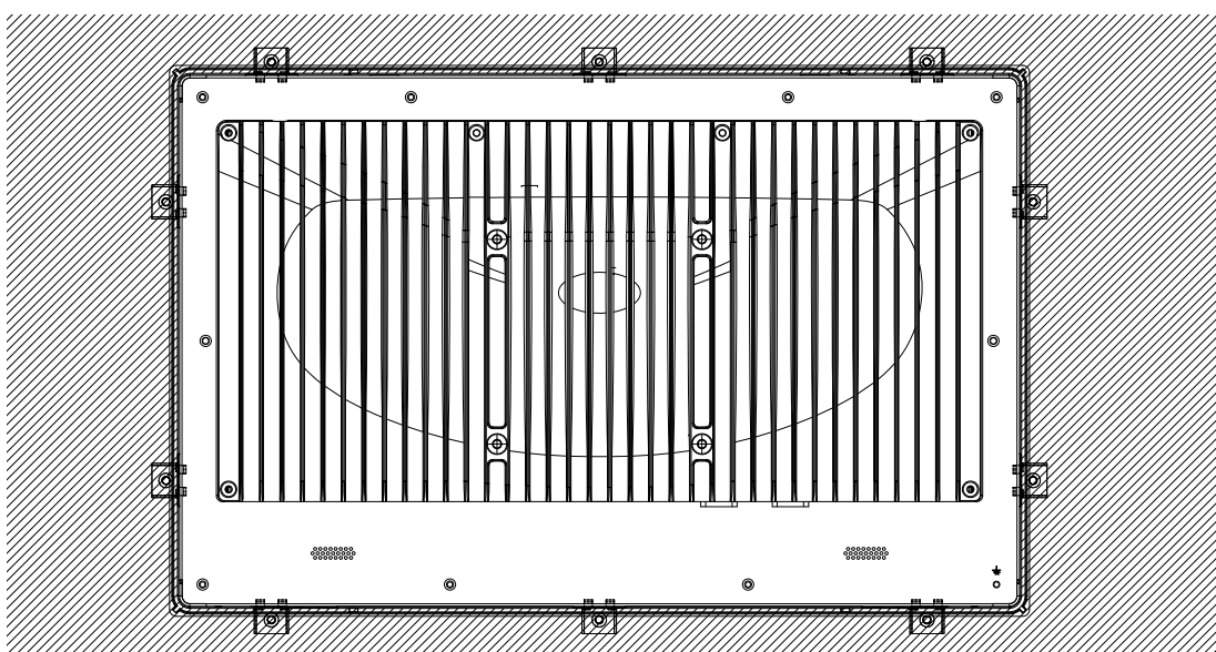
Figure 2.27 Panel mount rear view
