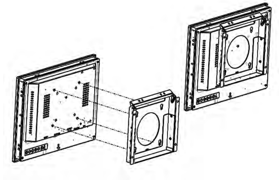
Figure 2.1 Wall Mounting
