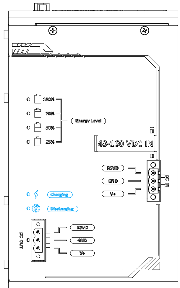
PB-9250J-110V
