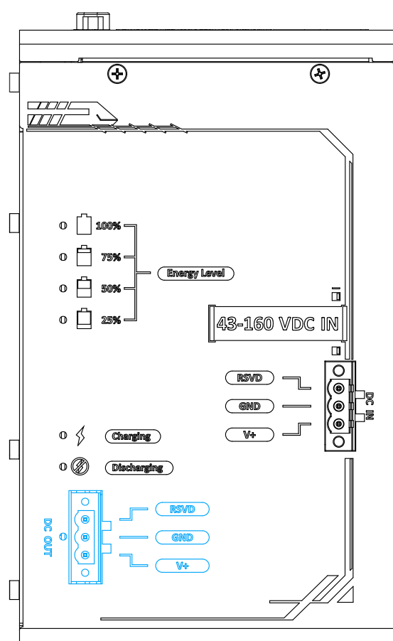
PB-9250J-110V
