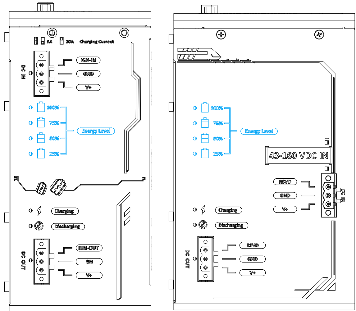
PB-9250/4600/2580
