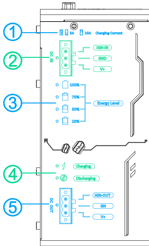
PB-9250/4600/2580
