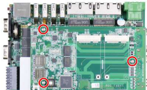
Secure MezIO module with screws
