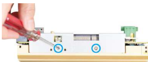
Remove the screws securing heat spreader
