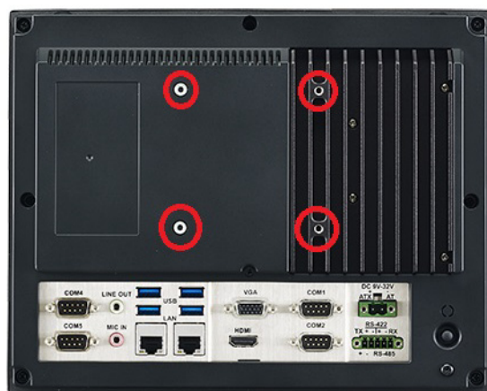
Figure 1.2 Rear Panel
