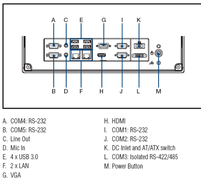
Figure 2.3 Panel PC I/O Ports
